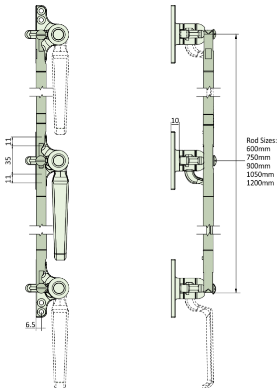
Dimensions Inward Opening 4-Hole Backplate
