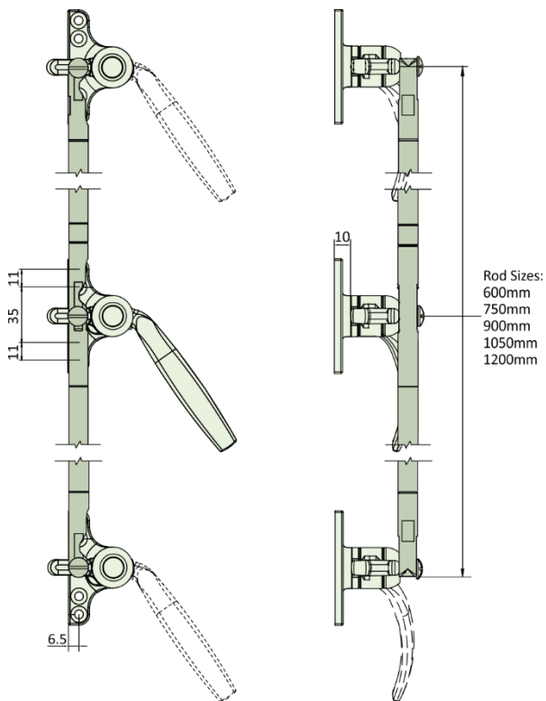
Dimensions Inward Opening In 4 hole Backplate Steel Window Fittings / Window Handles /B158/Triplex/OI
