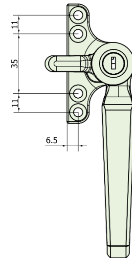
4-Hole Backplate Dimensions
